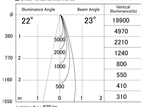
■ Direct Horizontal Illuminance DD155-0825DB9027
