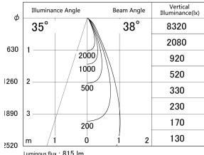
■ Direct Horizontal Illuminance DD155-0835DB9027
