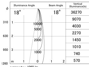
■ Direct Horizontal Illuminance DD155-1015DB9027
