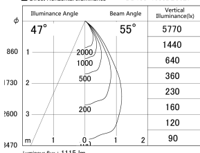
■ Direct Horizontal Illuminance DD155-1055DB9027
