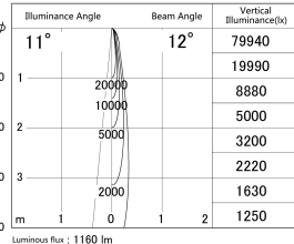
■ Direct Horizontal Illuminance DD155-1510DB9027
