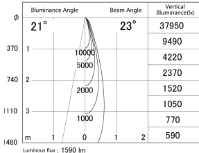
■ Direct Horizontal Illuminance DD155-1525DB9027
