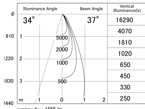
■ Direct Horizontal Illuminance DD155-1535DB9027
