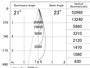
■ Direct Horizontal Illuminance DD155-2025DB9027
