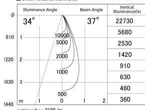
■ Direct Horizontal Illuminance DD155-2035DB9027
