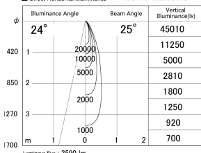
■ Direct Horizontal Illuminance DD155-2525DB9027
