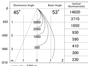
■ Direct Horizontal Illuminance DD155-2555DB9027
