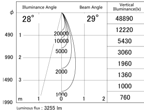
■ Direct Horizontal Illuminance DD155-3030DB9027
