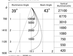
■ Direct Horizontal Illuminance DD155-3040DB9027
