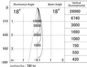
■ Direct Horizontal Illuminance DD155-0815DB9030
