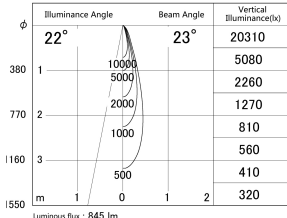
■ Direct Horizontal Illuminance DD155-0825DB9030
