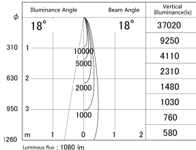
■ Direct Horizontal Illuminance DD155-1015DB9030
