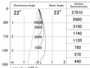
■ Direct Horizontal Illuminance DD155-1025DB9030
