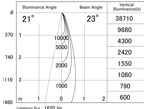
■ Direct Horizontal Illuminance DD155-1525DB9030
