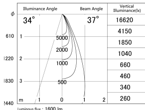
■ Direct Horizontal Illuminance DD155-1535DB9030
