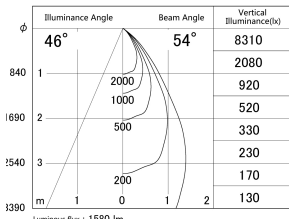
■ Direct Horizontal Illuminance DD155-1555DB9030
