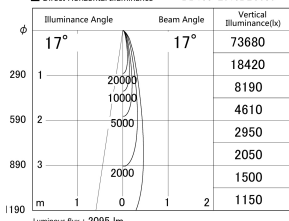
■ Direct Horizontal Illuminance DD155-2015DB9030
