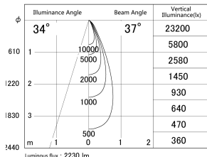
■ Direct Horizontal Illuminance DD155-2035DB9030
