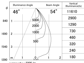
■ Direct Horizontal Illuminance DD155-2055DB9030
