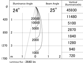
■ Direct Horizontal Illuminance DD155-2525DB9030
