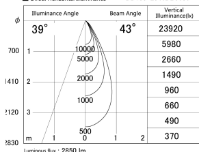
■ Direct Horizontal Illuminance DD155-2540DB9030
