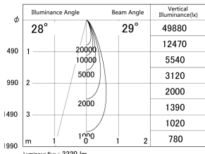
■ Direct Horizontal Illuminance DD155-3030DB9030
