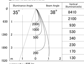
■ Direct Horizontal Illuminance DD155-0835DB9035
