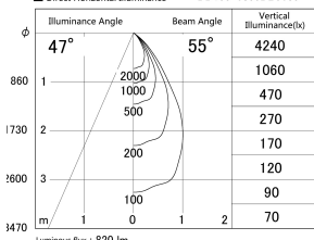
■ Direct Horizontal Illuminance DD155-0855DB9035
