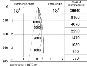
■ Direct Horizontal Illuminance DD155-1015DB9035
