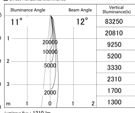
■ Direct Horizontal Illuminance DD155-1510DB9035
