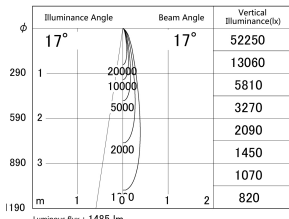
■ Direct Horizontal Illuminance DD155-1515DB9035
