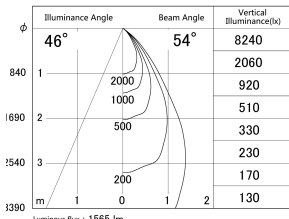
■ Direct Horizontal Illuminance DD155-1555DB9035
