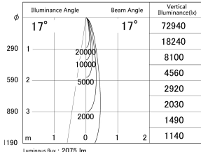
■ Direct Horizontal Illuminance DD155-2015DB9035
