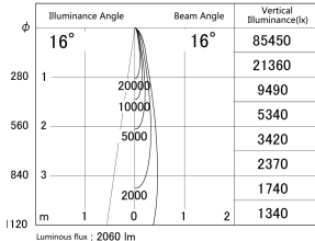
■ Direct Horizontal Illuminance DD155-2515DB9035
