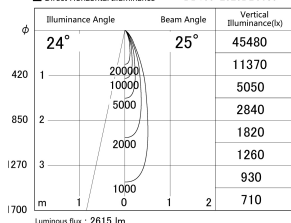
■ Direct Horizontal Illuminance DD155-2525DB9035
