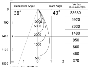
■ Direct Horizontal Illuminance DD155-2540DB9035
