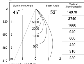
■ Direct Horizontal Illuminance DD155-2555DB9035
