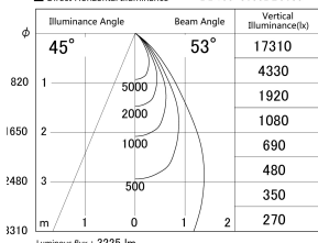
■ Direct Horizontal Illuminance DD155-3055DB9035
