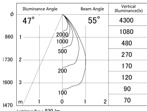
■ Direct Horizontal Illuminance DD155-0855DB9040
