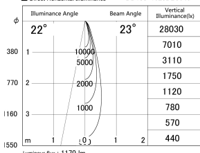
■ Direct Horizontal Illuminance DD155-1025DB9040
