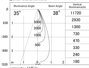
■ Direct Horizontal Illuminance DD155-1035DB9040
