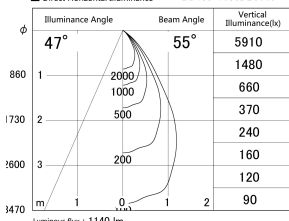
■ Direct Horizontal Illuminance DD155-1055DB9040
