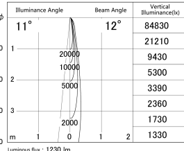
■ Direct Horizontal Illuminance DD155-1510DB9040
