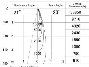
■ Direct Horizontal Illuminance DD155-1525DB9040
