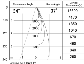
■ Direct Horizontal Illuminance DD155-1535DB9040
