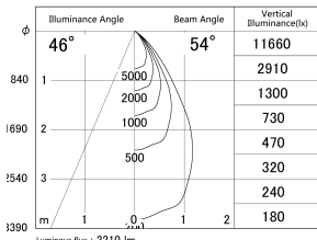
■ Direct Horizontal Illuminance DD155-2055DB9040
