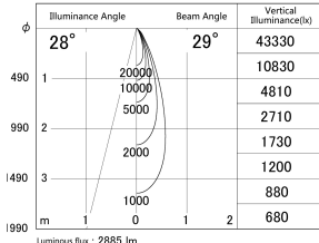
■ Direct Horizontal Illuminance DD155-2530DB9040
