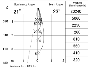
■ Direct Horizontal Illuminance DD155-0825WW9027
