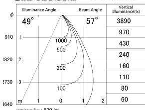
■ Direct Horizontal Illuminance DD155-0855WW9027
