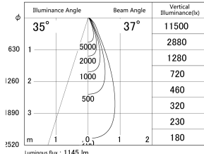
■ Direct Horizontal Illuminance DD155-1035WW9027
